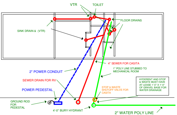
PLAN FOR SEWER, POWER, WATER, FOR INDIVIDUAL PADS
